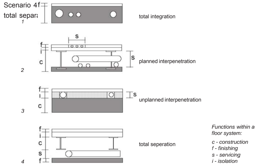
Figure 5.07: Levels of functional autonomy within a floor
