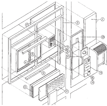
Figure 3.19: Levels of technical composition of one façade (Kapteijns 1998)
