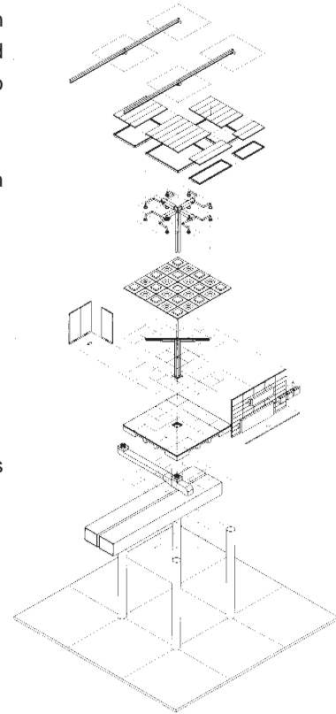
Diagram 3.1: Integration of building elements into a flexible structure (Addis 1994)
