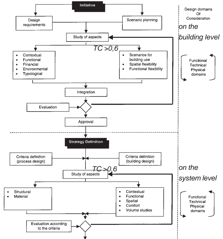
Integrated Design for Disassembly approach
