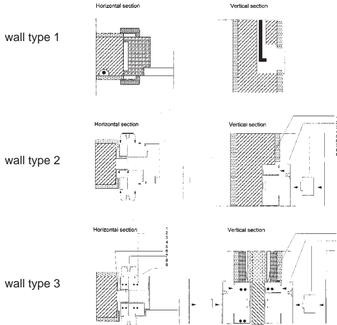
Figure 6.08: three types of wall systems: wall type 1- conventional wall Wall type 2 – conventional wall with separated zone for electrical components Wall type 3- flexible wall system with demountable components
