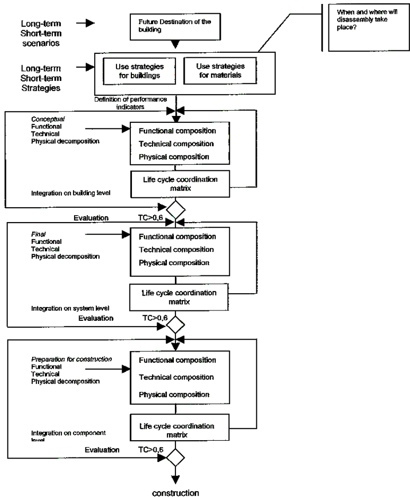
Figure 7.07 design scheme
