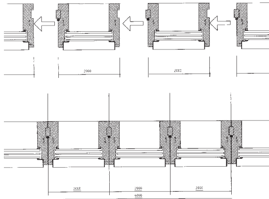
figure 5.39: Alternative configuration of the façade system of the XX building that has a higher disassembly potential of system components. Left assembly direction, right relational diagram
